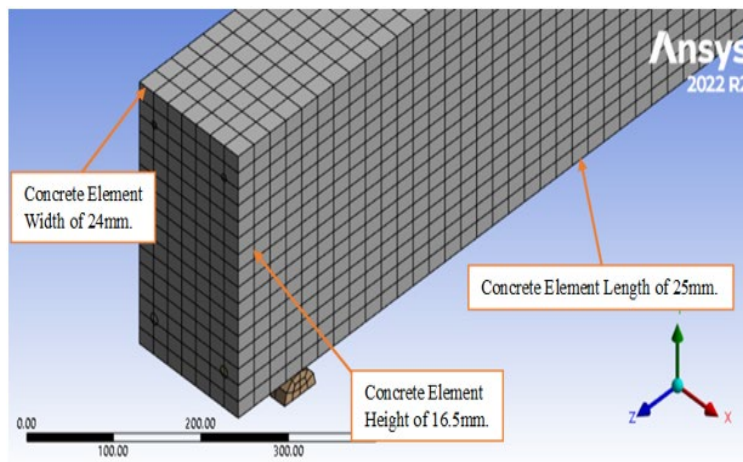
Fig. (5). The meshes of the numerical model in ANSYS
