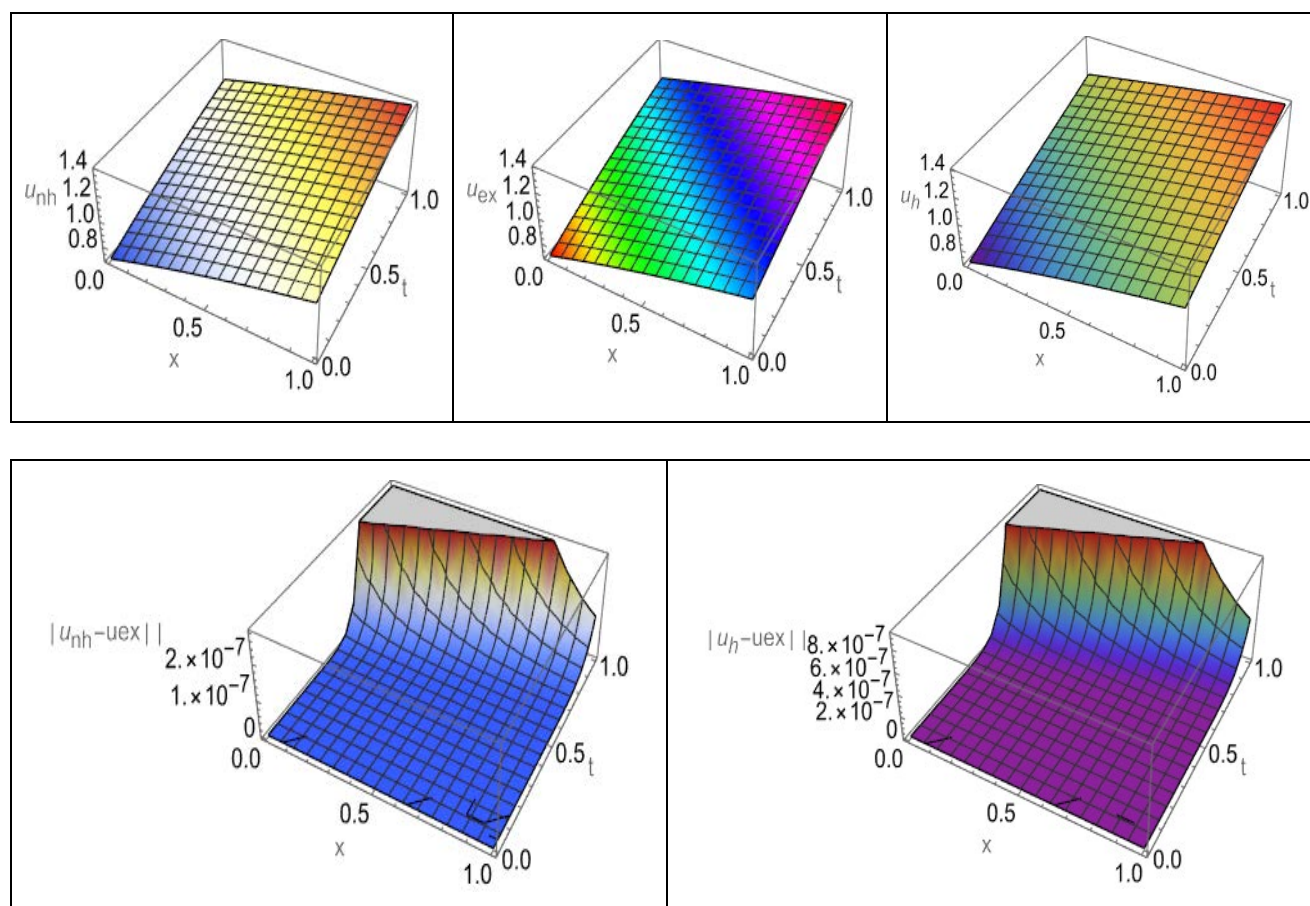
Figure: (4). Comparing between approximate solutions obtained via HPM, NHM, and exact solution on the interval (x, t) \in (0.1) \times [0,1] of ex.2
